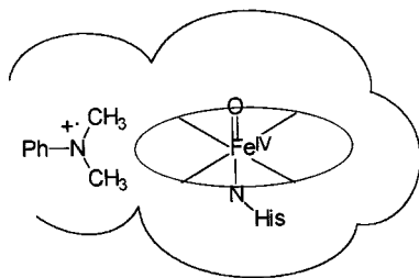
Figure 2. Rough visualisation of the heme-edge approach of N,N -dimethylaniline in the LiP active site
