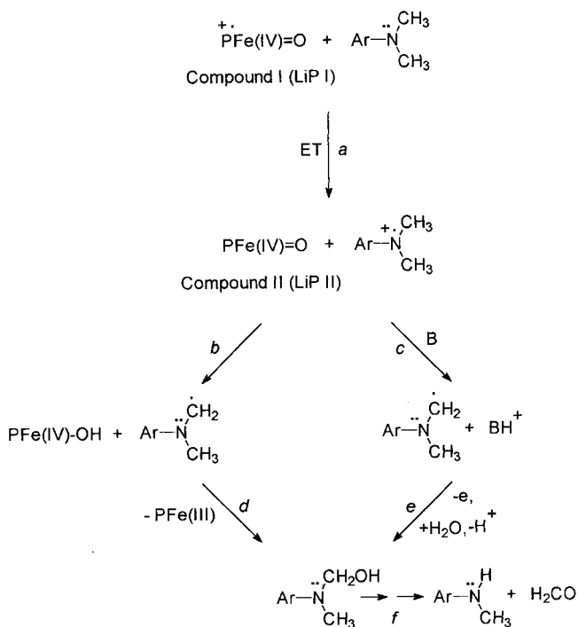
Scheme 1. Electron transfer mechanism for the oxidative N -demethylation of N,N -dimethylanilines catalysed by LiP
