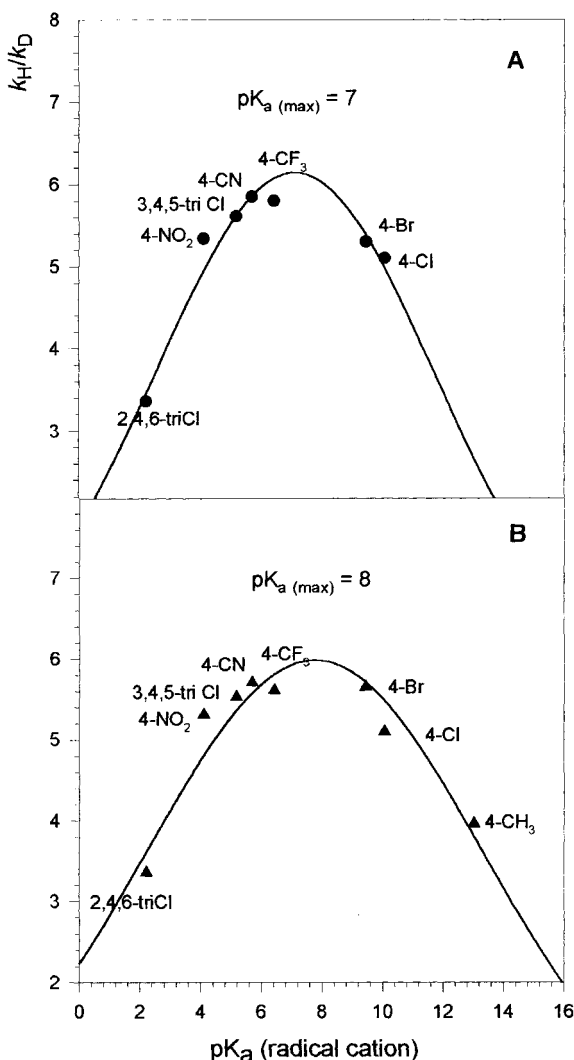
Figure 1. Bell-shaped curve for the LiP (A) and FeTPPSCI (B) catalysed oxidative N -demethylation of ring substituted N,N -bis(dideuteriomethyl)anilines
