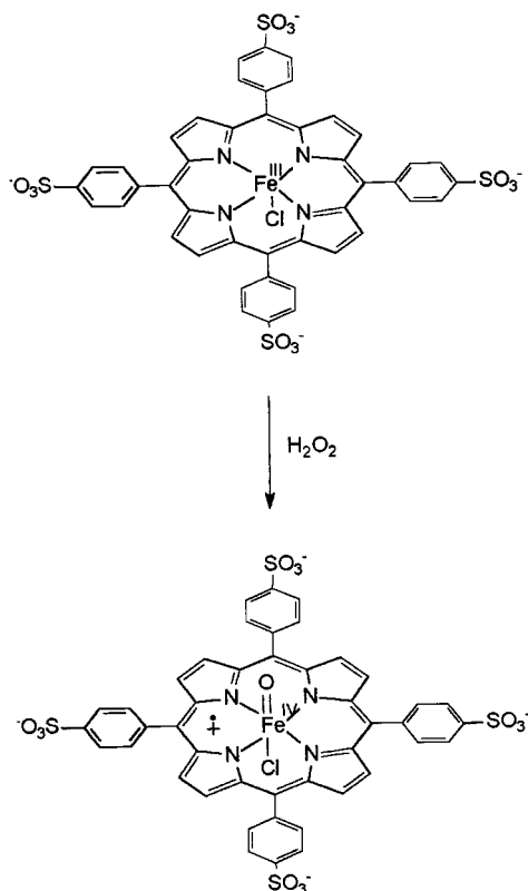
Scheme 3. Formation of the active oxidant by reaction of FeTPPS with H_2O_2
