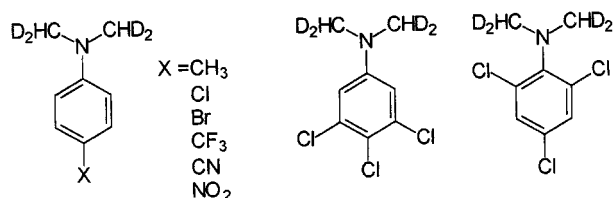
Scheme 2. Ring substituted N,N -bis(dideuteriomethyl)anilines used in this work
